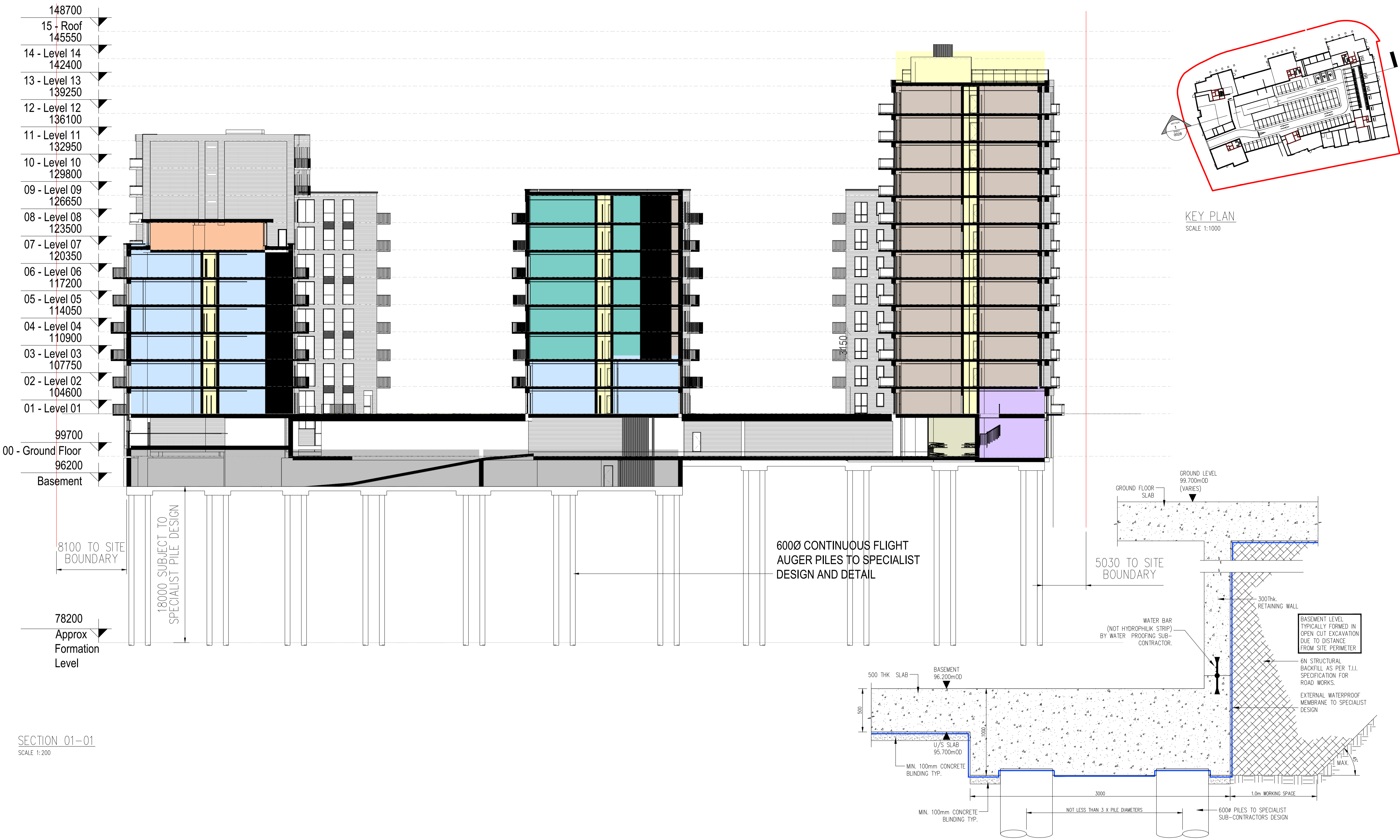
TYPICAL SUB-STRUCTURE DETAIL SCALE 1:20
